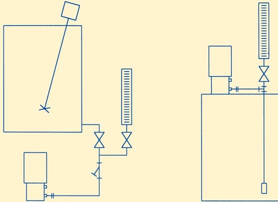
PUMP SUCTION-FLOODED
